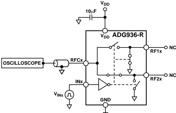
Figure 24. Video Feedthrough
